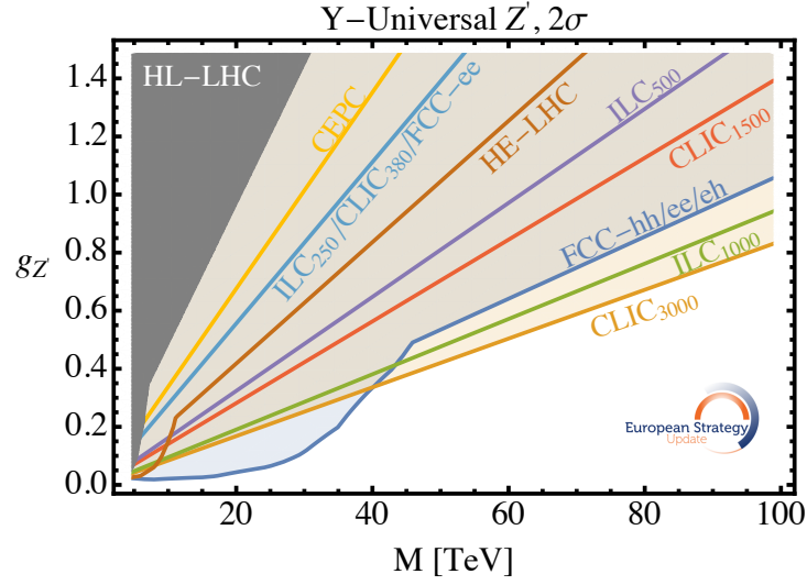
Fig. 8.3: Exclusion reach of different colliders on the Y -Universal Z' model parameters. The gap in performances between CEPC or FCC-ee with respect to ILC 250 or CLIC 380 is most likely due to the lack of dedicated di-fermion production studies as discussed in Sect. 8.2.1.
