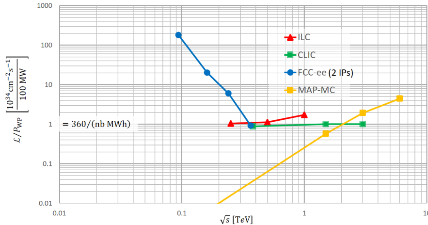
Fig. 10.7: One possible figure of merit for future colliders: luminosity per supplied primary energy (from E. Jensen and M. Seidel's presentation in Granada [682]).
