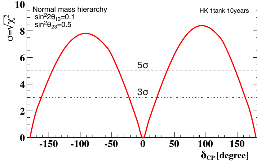
Fig. 6.4: Hyper-Kamiokande expected significance to exclude \sin \delta_{CP} = 0 in case of normal hierarchy [375] for an exposure of 10 years. The mass ordering is assumed to be known.
