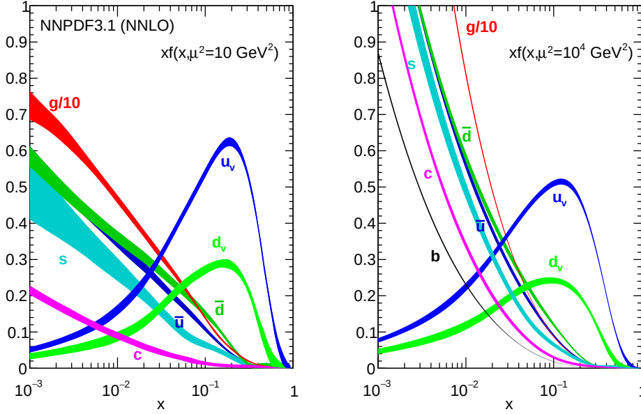
Fig. 4.4: Different PDFs as obtained at NNLO level (NNPDF3.1) from Ref. [168], evaluated at \mu^2 = 10 \text{ GeV}^2 (left) and \mu^2 = 10^4 \text{ GeV}^2 (right).
