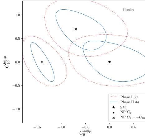
Fig. 5.9: Combined sensitivity of LHCb, ATLAS and CMS after the HL-LHC phase to potential new physics in b \rightarrow s\mu\mu processes, motivated by recent anomalies (from Ref. [302]). New physics benchmarks with leptonic vector current (new physics only in C_9 ) or pure left-handed current ( C_9 = -C_{10} ), as well as the SM predictions are shown. The observables included are the branching ratio of the B_s \rightarrow \mu^+\mu^- decay and the angular observables of the decay B^0 \rightarrow K^{*0}\mu^+\mu^- in the low- q^2 region. See Ref. [302] for details.
