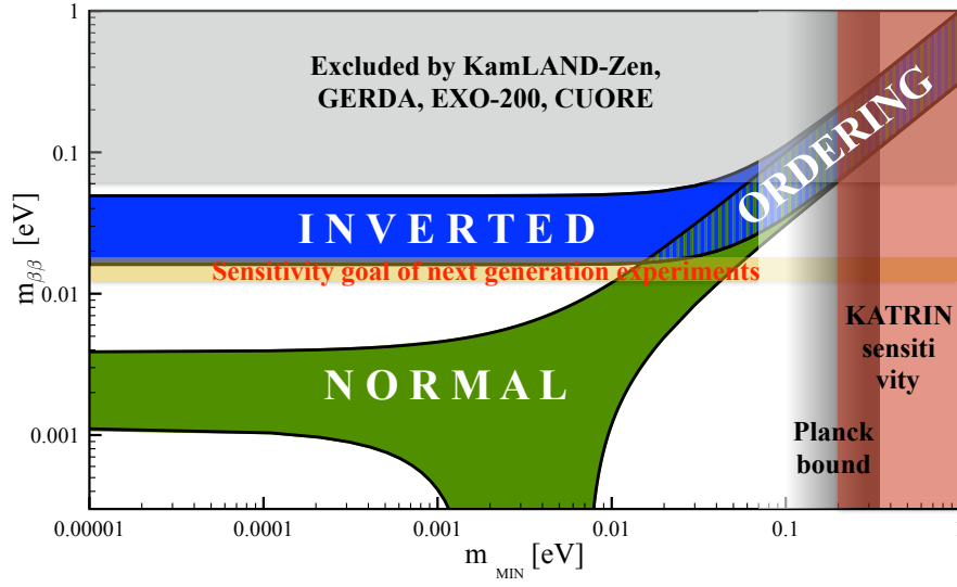
Fig. 6.5: The effective mass m_{\beta\beta} controlling the rate of the neutrino-less double beta decay versus the mass of the lightest eigenstate [381]. The limits from the current and future experiments are shown.
