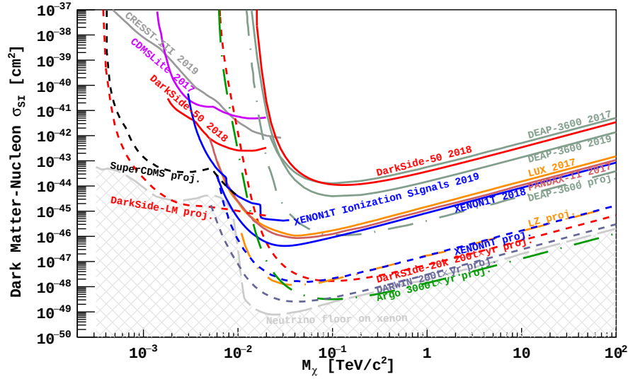
Fig. 9.1: 90% CL exclusion limits showing leading results from direct detection (continuous lines, Refs. [535, 536, 541, 544–546]). Sensitivities of future Ge-, Xe-, and Ar-based direct searches are also shown with dashed lines, Ref. [547–551]). The neutrino floor curve follows the definition of Refs. [552].
