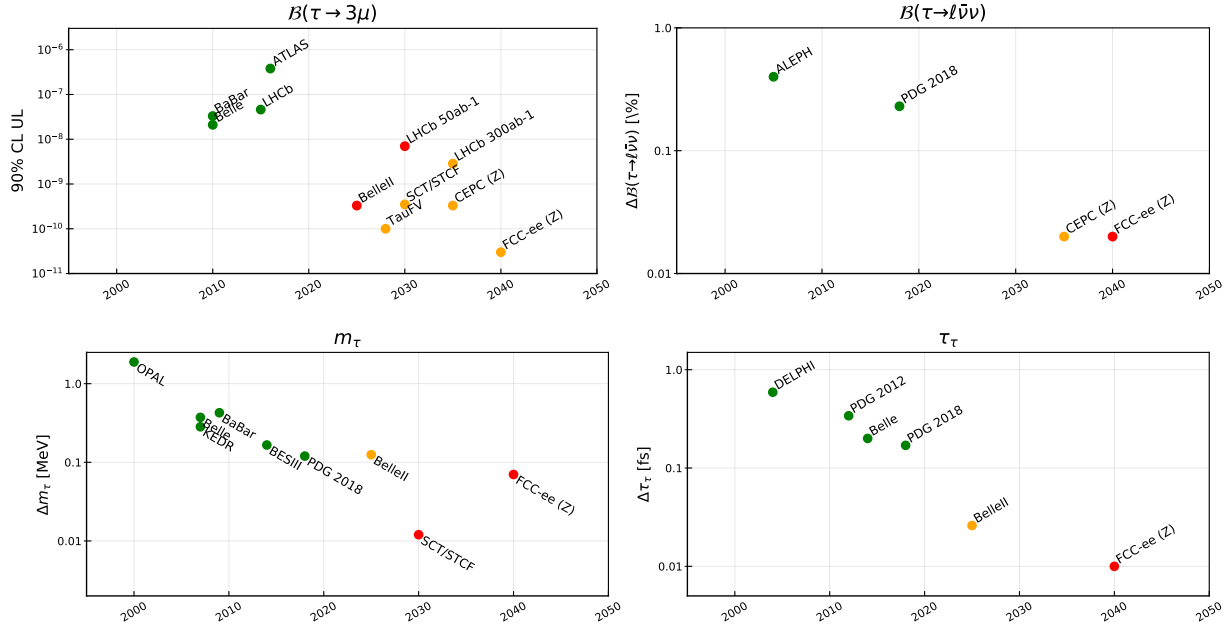
Fig. 5.11: Expected sensitivity and projected precision of present and future experiments for \tau \rightarrow 3\mu , \tau \rightarrow \ell \bar{\nu} \nu decays, m_\tau and \tau_\tau [331]. Green denotes current measurements, red points correspond to estimates of future experimental sensitivities based on dedicated studies (relying on extrapolation from past established performances) while orange corresponds to estimates of experimental sensitivities including novel features (for which extrapolation from past experience is more difficult).
