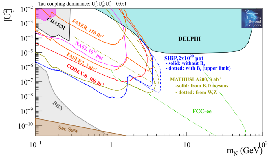
Fig. 5.13: Reach of proposed experiments for heavy neutral leptons coupling predominantly to the tau flavour (from Ref. [354]), while for electron and muon flavours they are given in Figs. 8.19 and 9.6, respectively. For Higgs mixed scalar the reach is given in Fig. 8.17.
