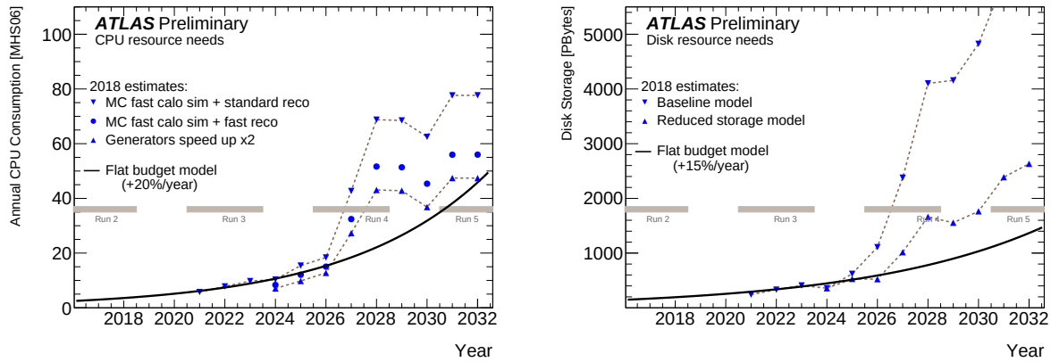
Fig. 11.2: Estimated CPU (left) and total disk resources (right) needed by the ATLAS experiment as a function of time for both data and simulation processing. Plots taken from [725].
