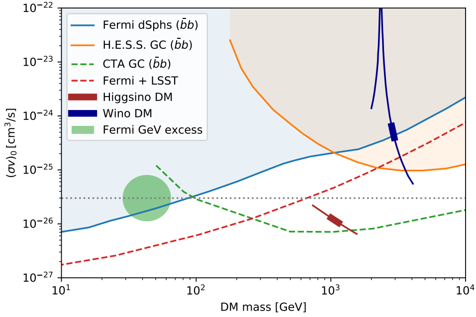
Fig. 9.2: Current constraints on the DM self-annihilation cross section into \bar{b}b from Fermi LAT (dSph) [556] and H.E.S.S. Galactic Centre (GC) [557], and expected future reach with the CTA and additional dwarfs found by LSST [558]. Also shown as red (blue) lines the annihilation cross sections for pure Higgsino (Wino) DM in the vicinity of DM masses yielding the correct relic density (the thick regions indicating the correct relic density, from [559]), as well as the parameter range preferred by the Fermi GeV excess [556,560]. The H.E.S.S. constraints weaken significantly if the DM profile at the Galactic centre is cored, leaving pure Wino DM consistent with H.E.S.S. and Fermi observations (see text for details).
