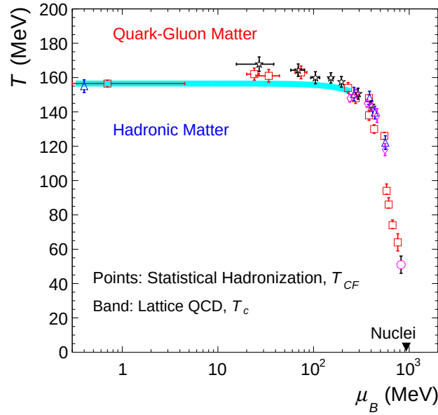
Fig. 4.2: The QCD phase diagram in the temperature – baryochemical potential plane. The band is from LQCD calculations [123], the points from statistical hadronisation model fits to hadron yields in heavy-ion collisions over a broad range of collision energy (updated from Ref. [111]).
