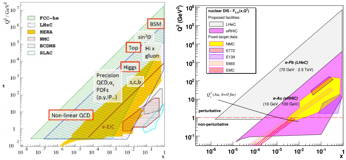
Fig. 4.1: Kinematic (x, Q^2) plane probed in e-p (left) and e-A processes (right): existing data compared to proposed particle and nuclear DIS facilities [114, 115].
