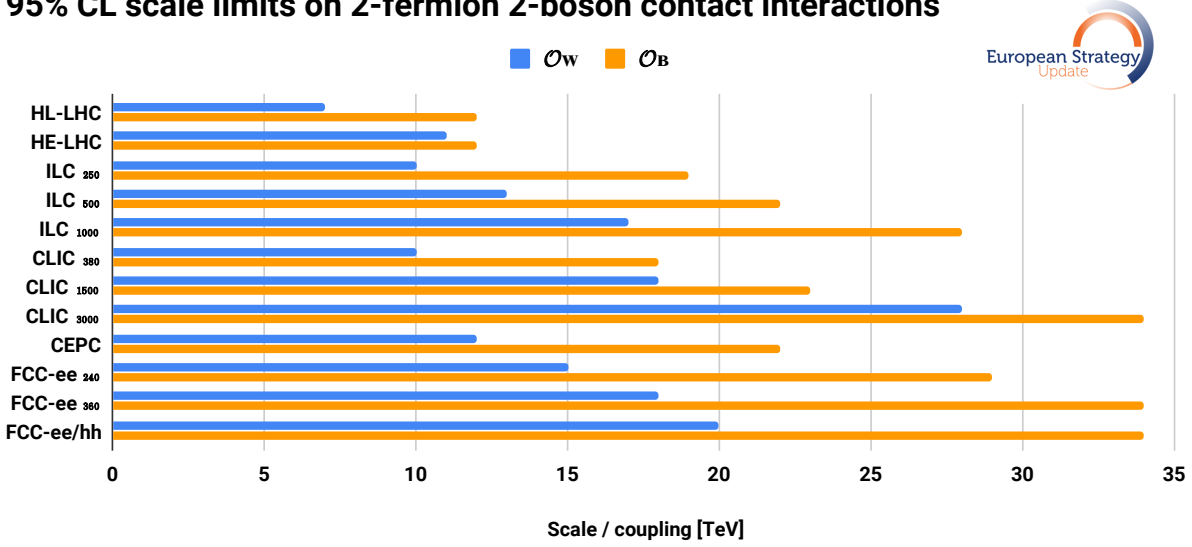
Fig. 8.2: Exclusion reach of different colliders on the two-fermion/two-boson contact interactions from the operator \mathcal{O}_W and \mathcal{O}_B . The blue bars give the reach on the effective scale \Lambda/(g_2^2\sqrt{c_W}) and the orange bars on \Lambda/(g_1^2\sqrt{c_B}) , where c_{W,B} are the Wilson coefficients of the corresponding operators and the gauge couplings come from the use of the equations of motion.
