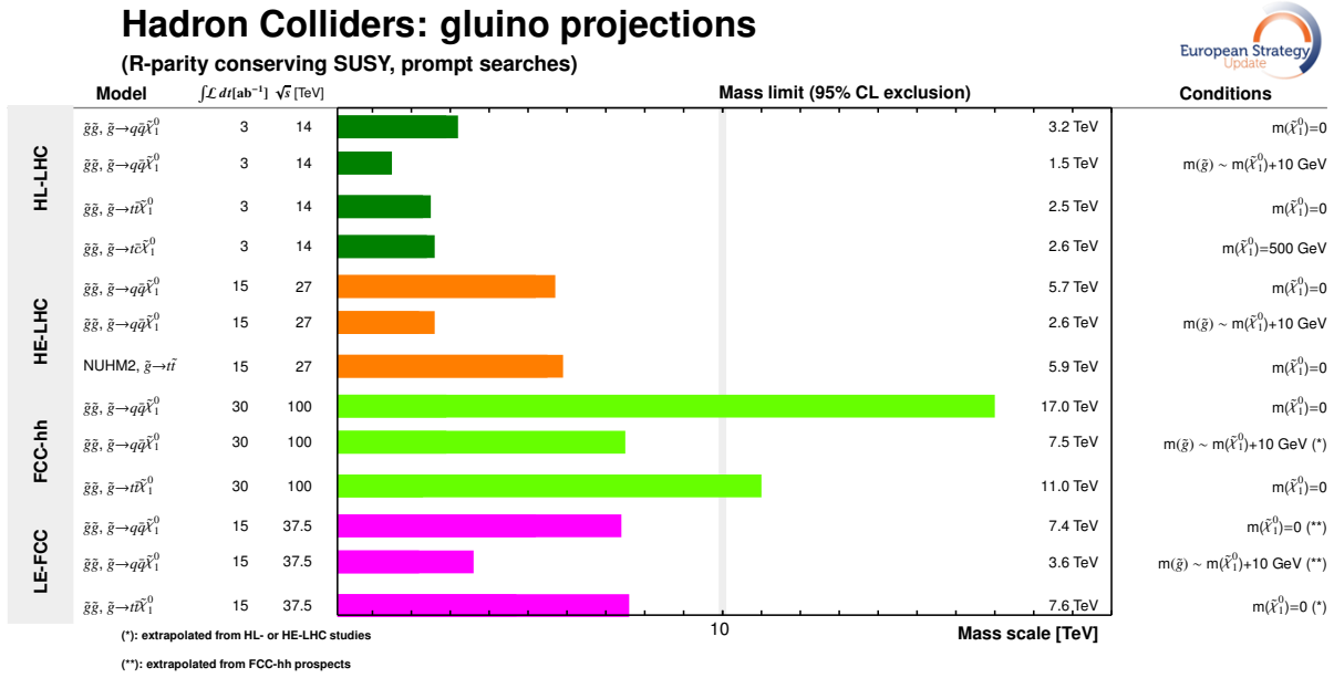
Fig. 8.6: Gluino exclusion reach of different hadron colliders: HL- and HE-LHC [436], and FCC-hh [134,441]. Results for low-energy FCC-hh are obtained with a simple extrapolation.
