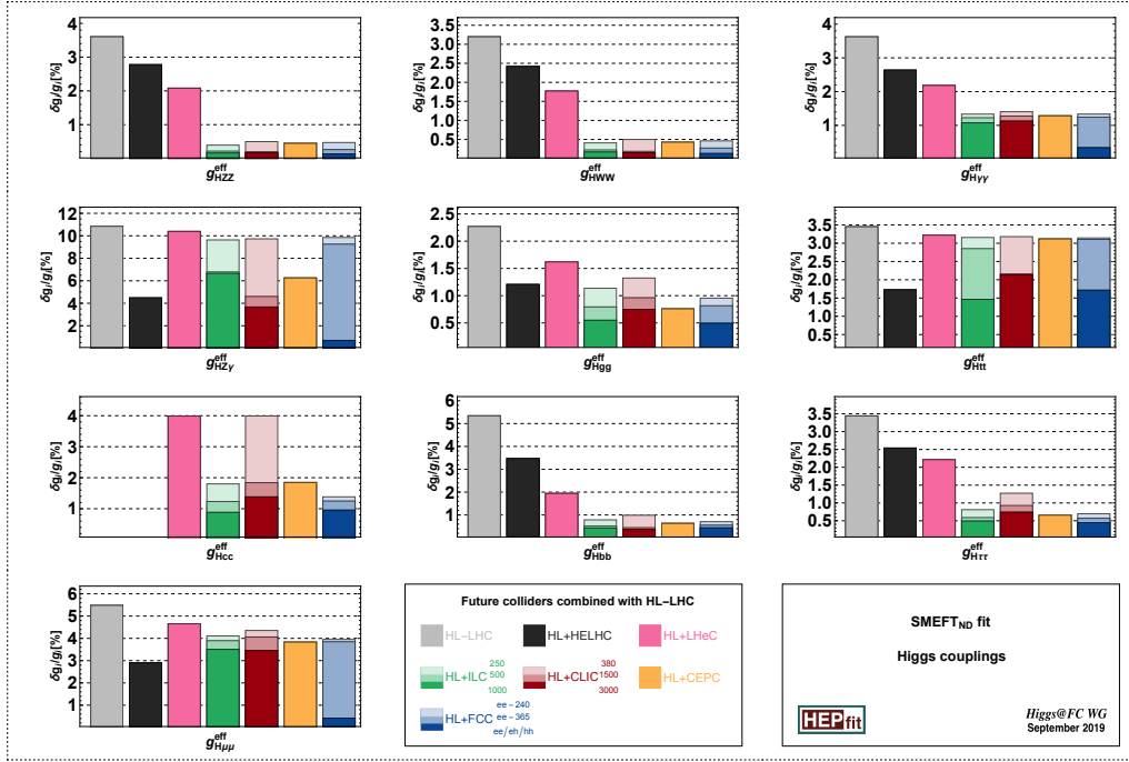
Fig. 3.9: 68% probability reach on Higgs couplings and aTGC at the different future colliders from the Global fit \text{SMEFT}_{\text{ND}} . For details, see Ref. [39].
