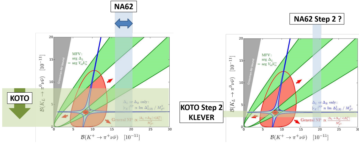
Fig. 5.5: Educated guess for the future of the K \rightarrow \pi \bar{\nu} \nu decays (shaded vertical and horizontal regions): mid and long-term (respectively left and right panels) [279]. Original figure from Ref. [292]: the red region illustrates the lack of correlation for NP models with general left-handed and right-handed couplings; in green the correlation present in some MFV models; in blue the correlation induced by the constraint from \epsilon_K if only left- or right-handed couplings are present.
