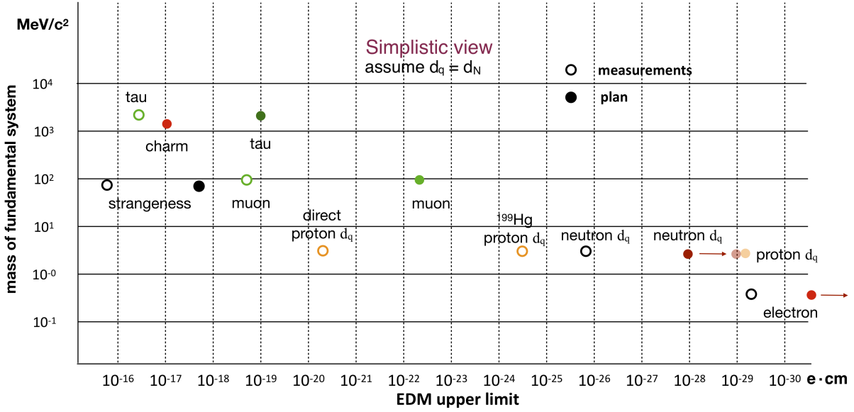
Fig. 5.3: Summary of current EDM limits (empty circles) and short/mid-term planned sensitivities (full circles) for light quarks, strange and charm quarks, electron, muon and tau [259].
