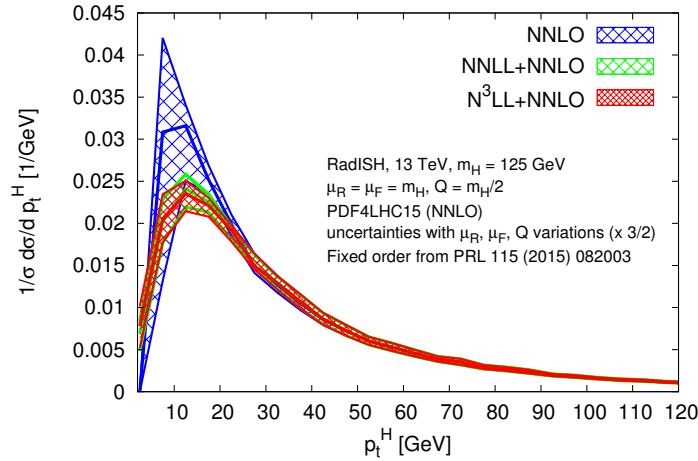
Fig. 4.3: Comparison among the matched normalised distributions at: N^3LL+NNLO , NNLL+NNLO , and the pure NNLO of the Higgs-boson transverse-momentum spectrum at the LHC [141].
