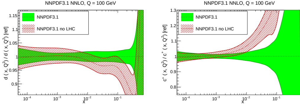
Fig. 4.5: The impact of the LHC data on the NNPDF3.1 NNLO PDFs for the down and charm quarks [168].
