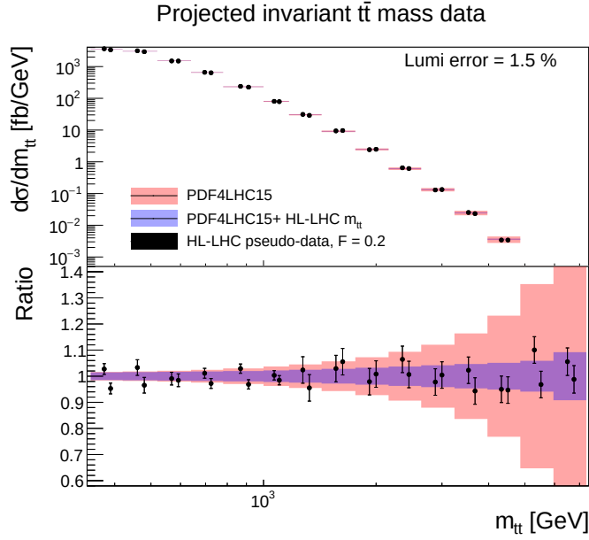
Fig. 4.6: Comparison between HL \tilde{\text{LHC}} pseudodata and the theoretical predictions for the m_{t\bar{t}} distribution in top quark pair production from Ref. [104]. The theory calculations are shown both before (PDF4LHC15) and after (PDF4LHC15-HL LHC) constraining PDFs with pseudodata in the fit.
