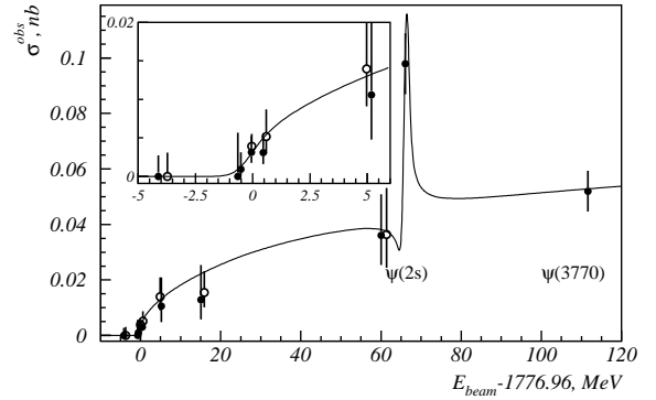
Figure 2. The measured cross section of e^+e^- \rightarrow \tau^+\tau^- versus center-of-mass energy and the fit. Just for illustration the additional data points (open circles) are corrected to the difference of detection efficiencies and shifted in energy to avoid overlap.
