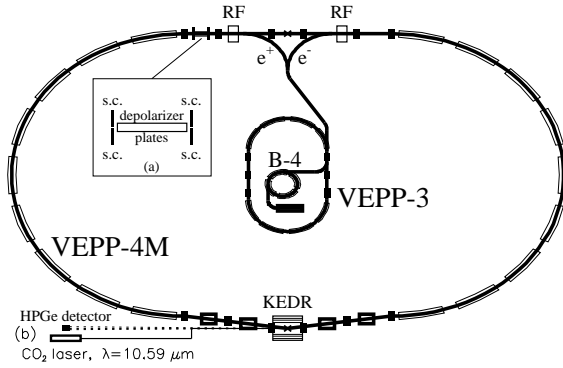
Figure 1. VEPP-4M accelerator complex in the energy calibration mode: (a) – Touschek polarimeter, (b) – Compton backscattering monitor.
